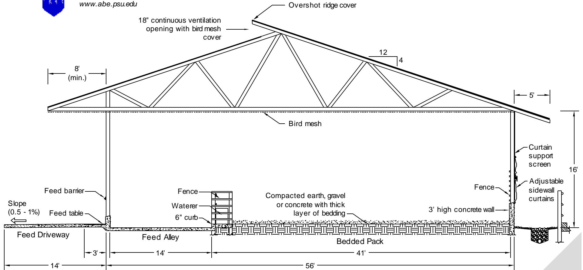
Gable Roof 1 Cross Section 2
