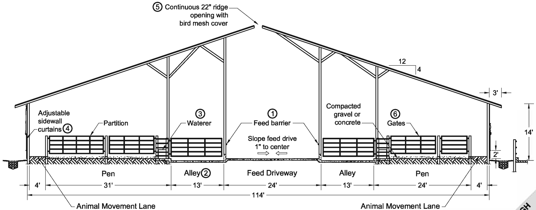
Post and Beam Roof Cross Section 1 2
