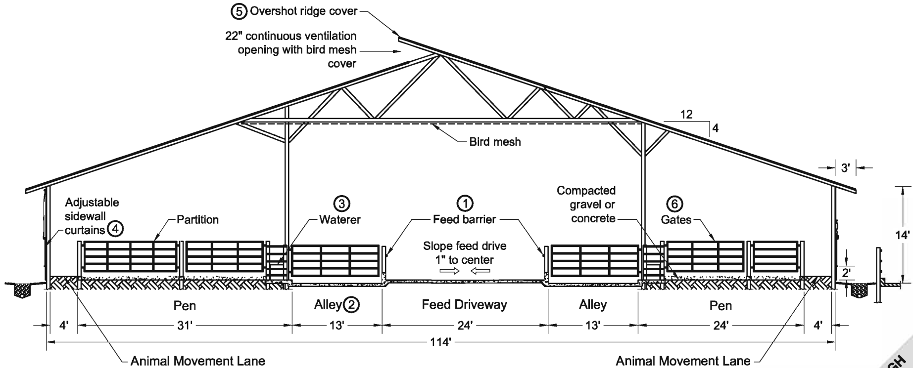
Truss Roof 1 Cross Section 3
