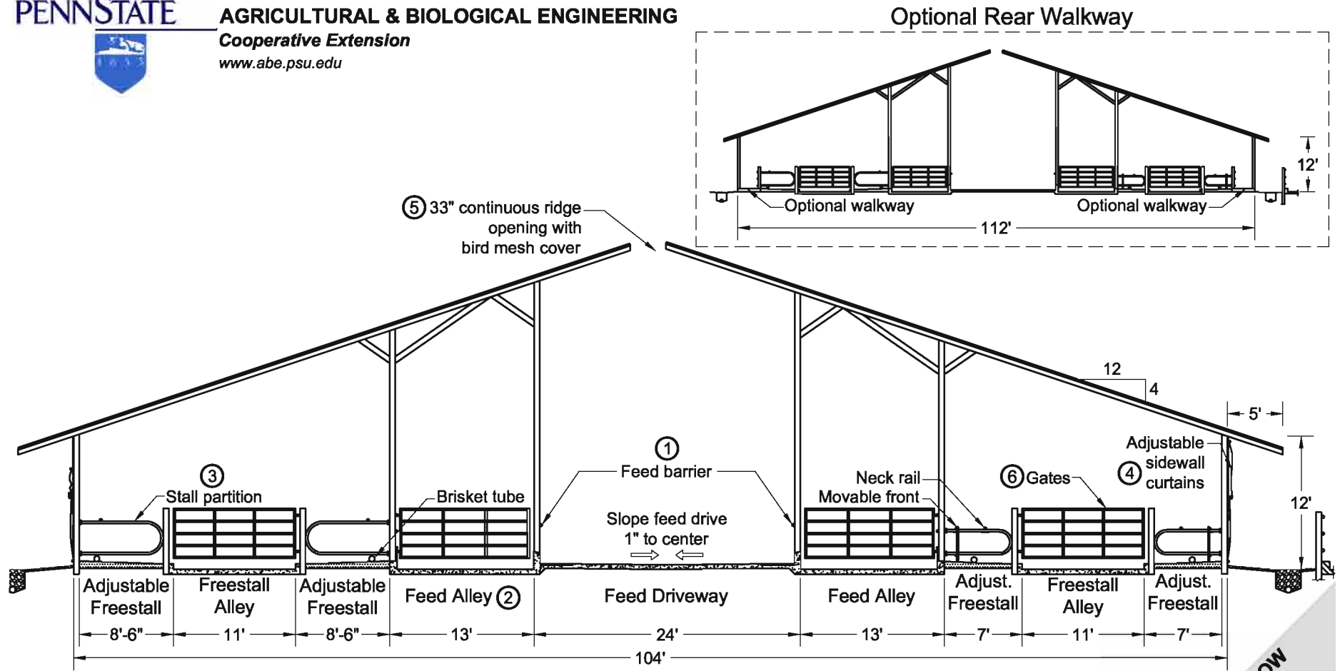
Post and Beam Roof 1 Cross Section 2
