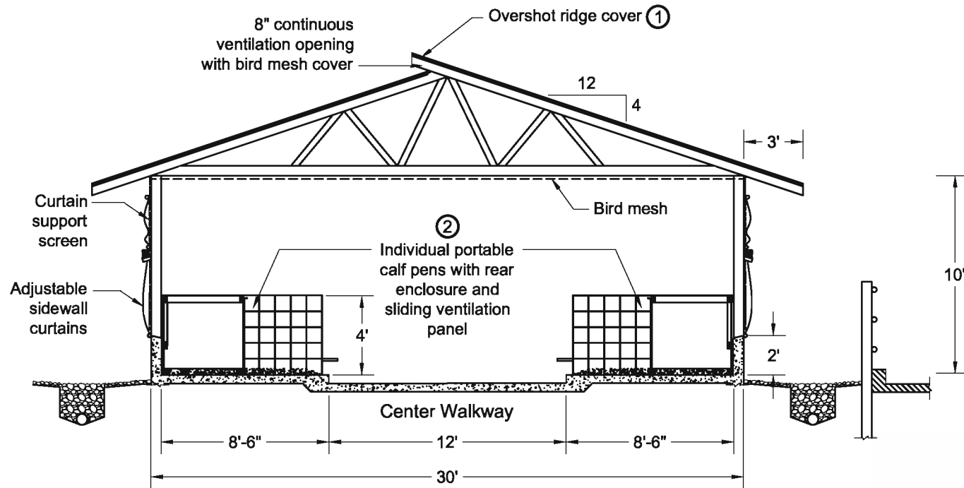
Calf Pens 1 Cross Section 2
