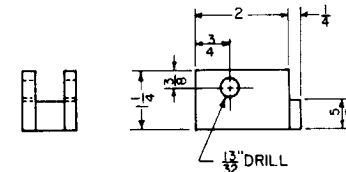
HINGE DETAILS
