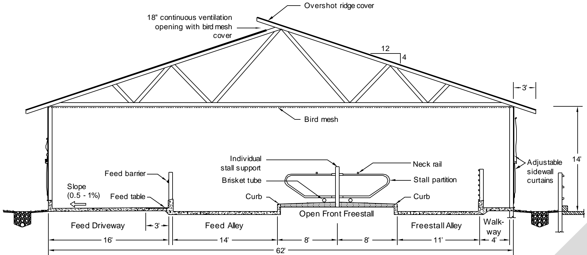
Gable Roof Cross Section with Freestall
