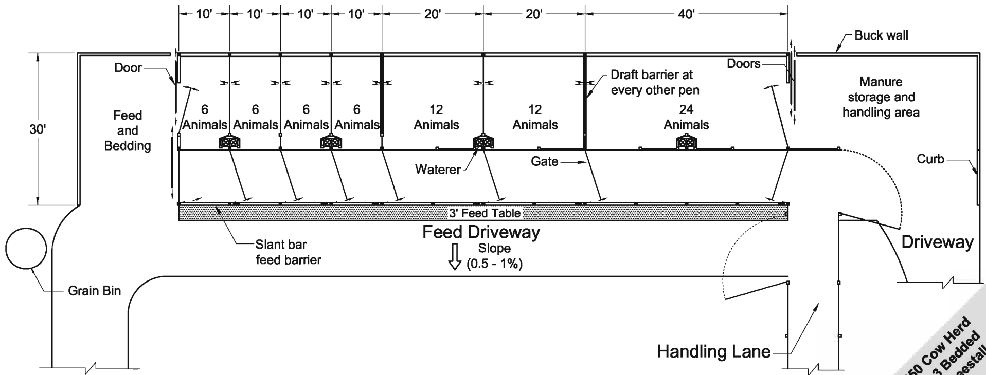
Weaned Calf Shelter 1 4 Plan View
