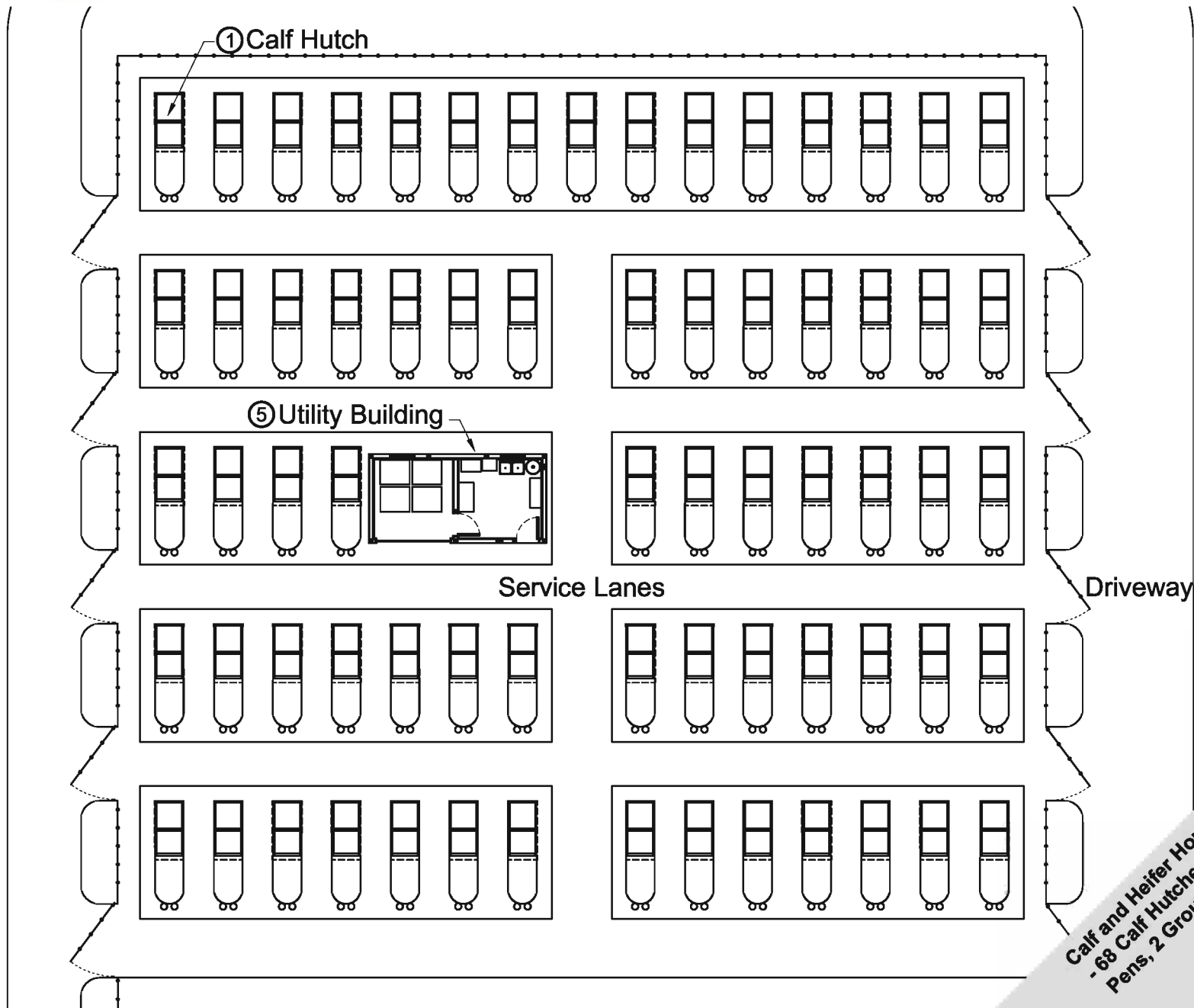
Calf Hutches 1 3 Plan View
