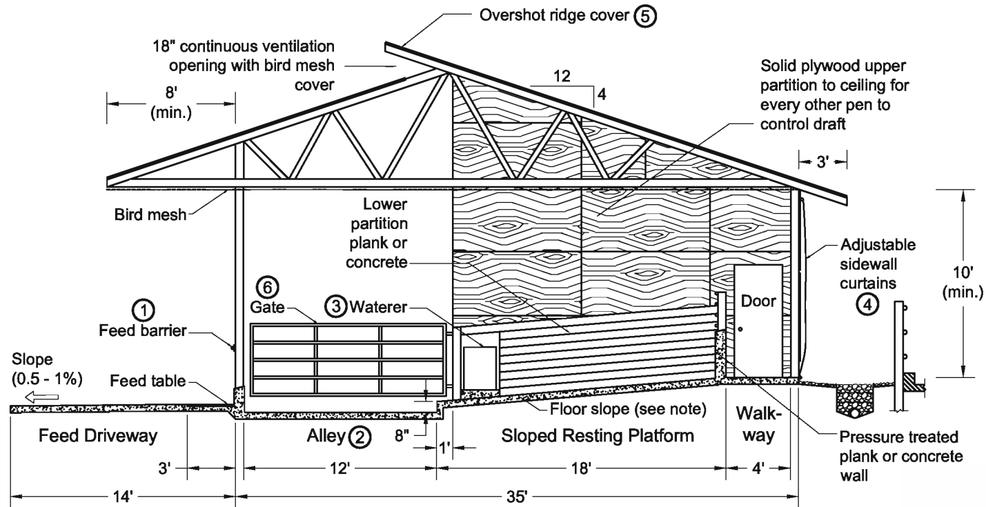
Gable Roof Cross Section with Concrete Alley (1/3)
