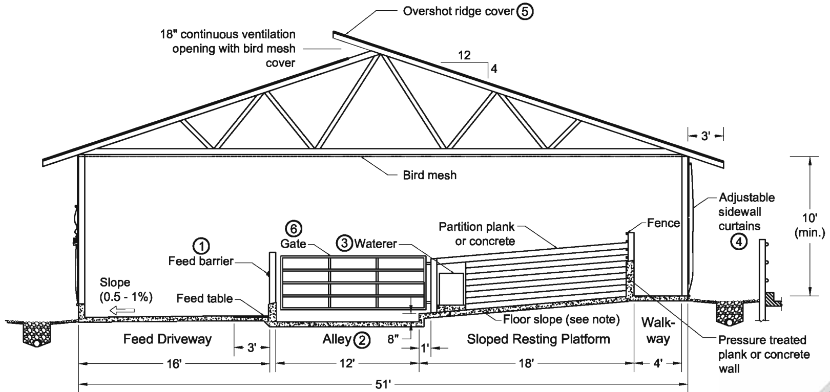
Gable Roof Cross Section, Inside Feeding 1 4
