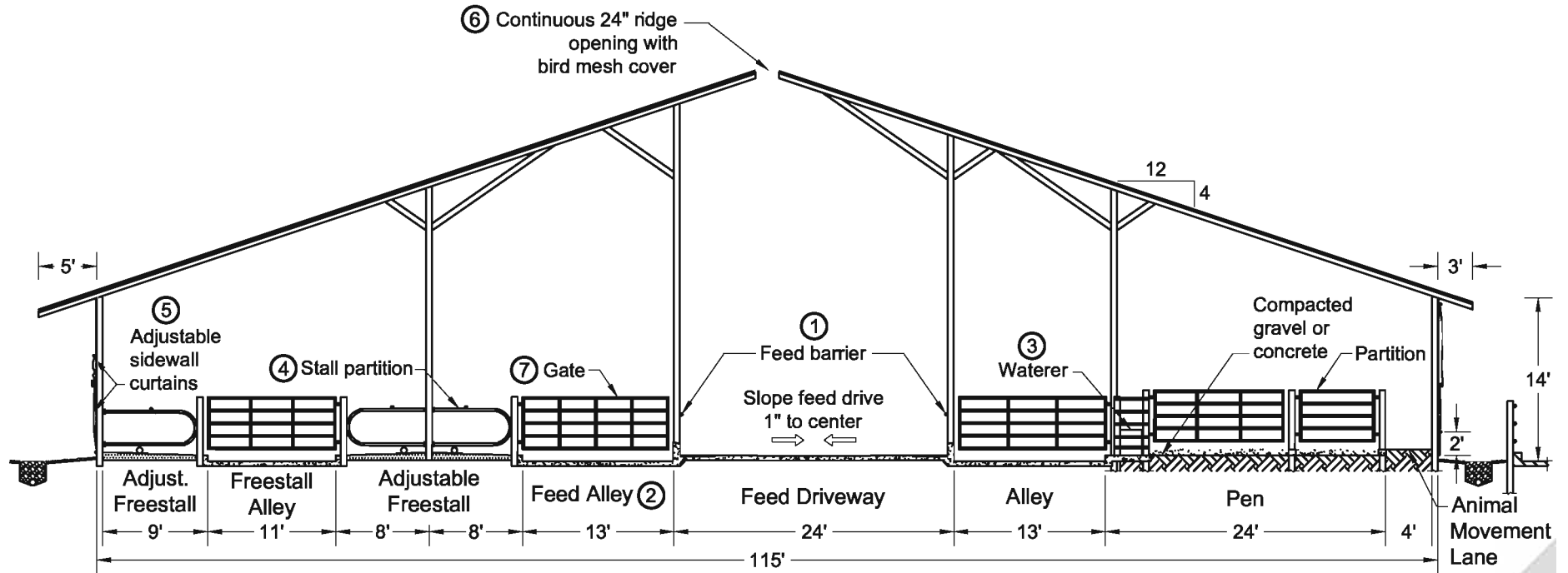
Post and Beam Roof 1 2 Cross Section
