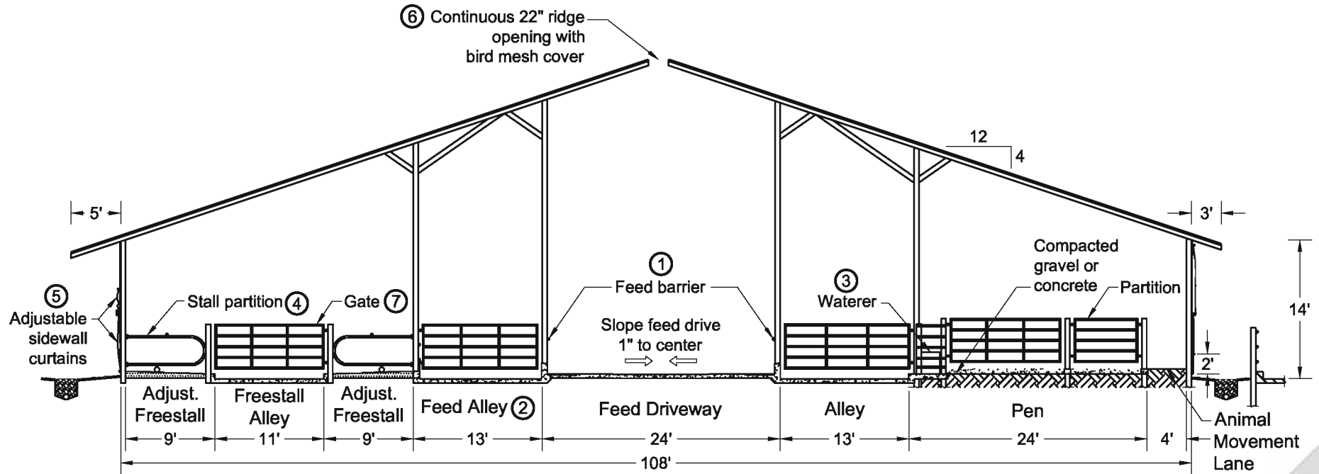
Post and Beam Roof Cross Section 1 2
