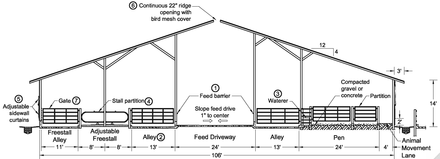
Post and Beam Roof 1 Cross Section 2
