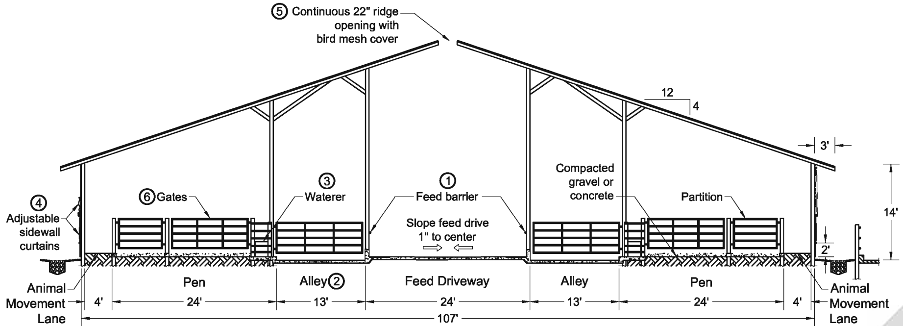
Post and Beam Roof Cross Section
