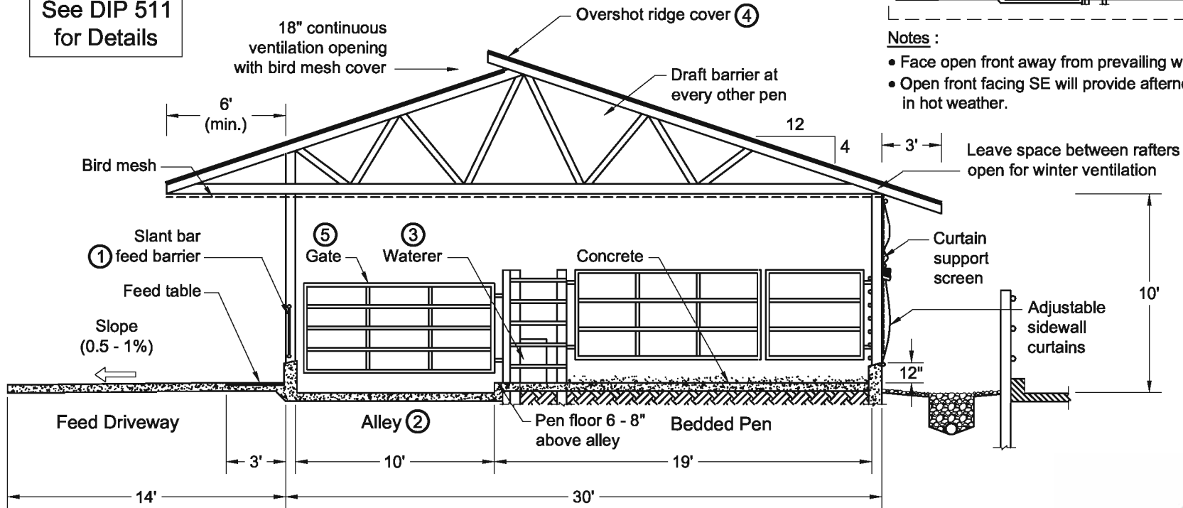
Weaned Calf Pen 1 Cross Section 3
