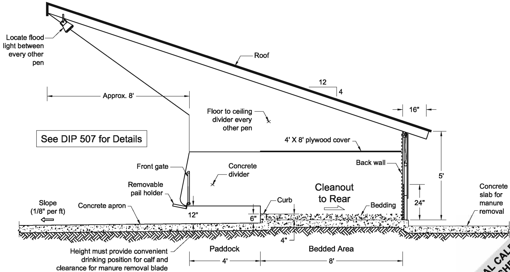
Individual Pen Detail 1 Cross Section 2
