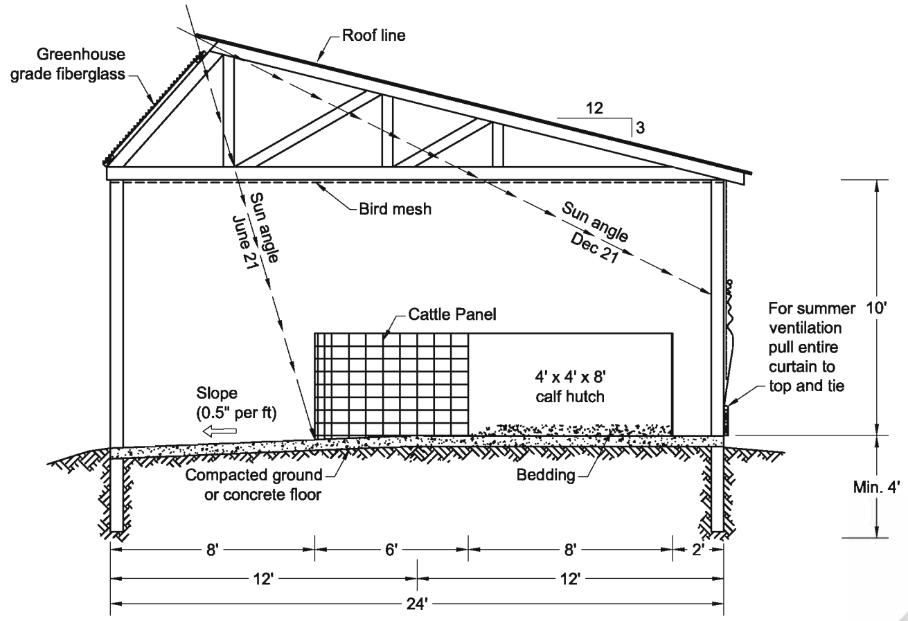
Truss Roof 1 Cross Section 3
