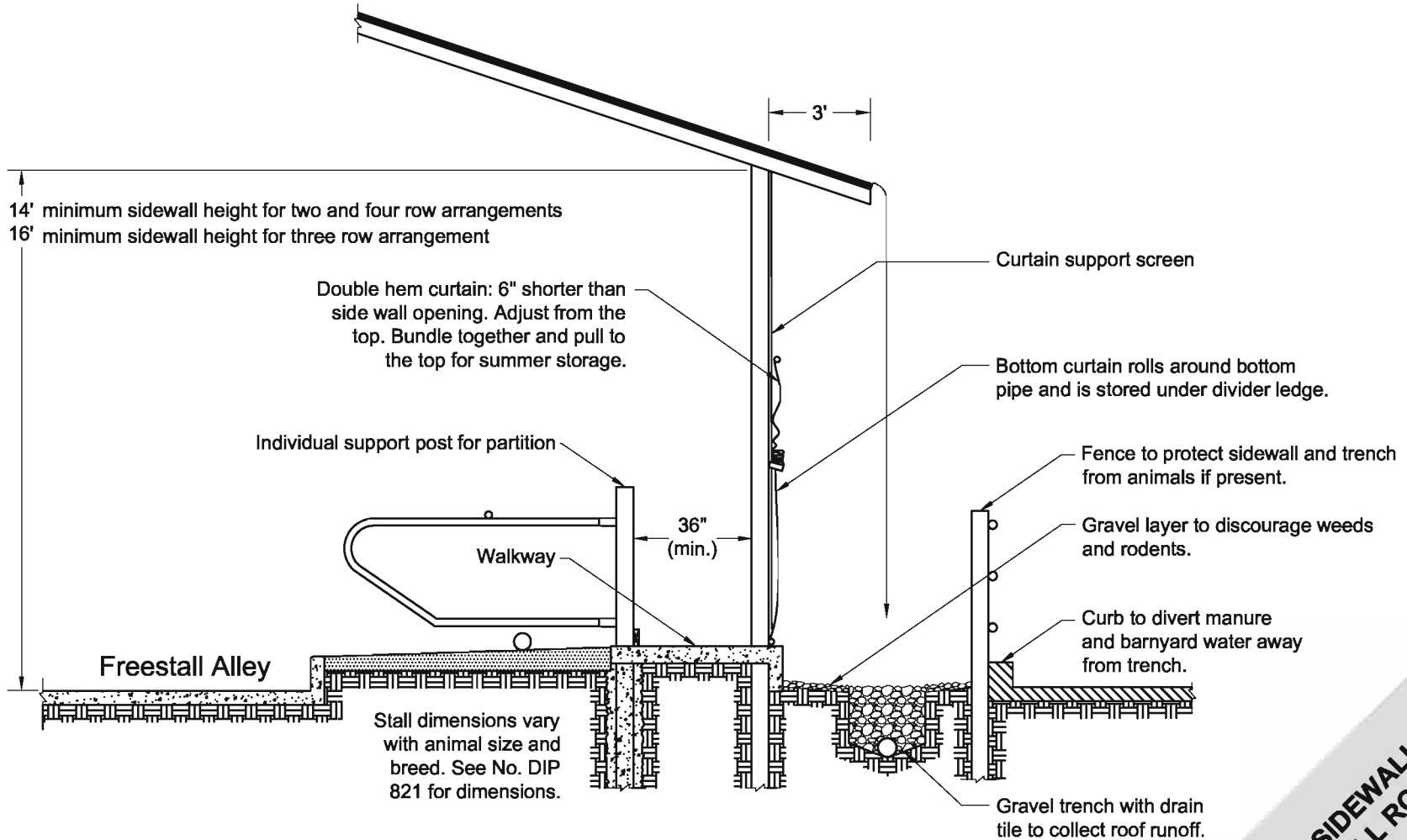
Freestall Wall with Rear Walkway
